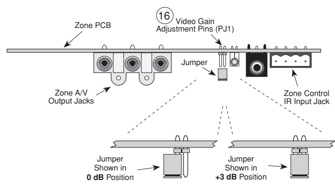
Fig. 4 Video Gain Adjustment - Jumper Locations
