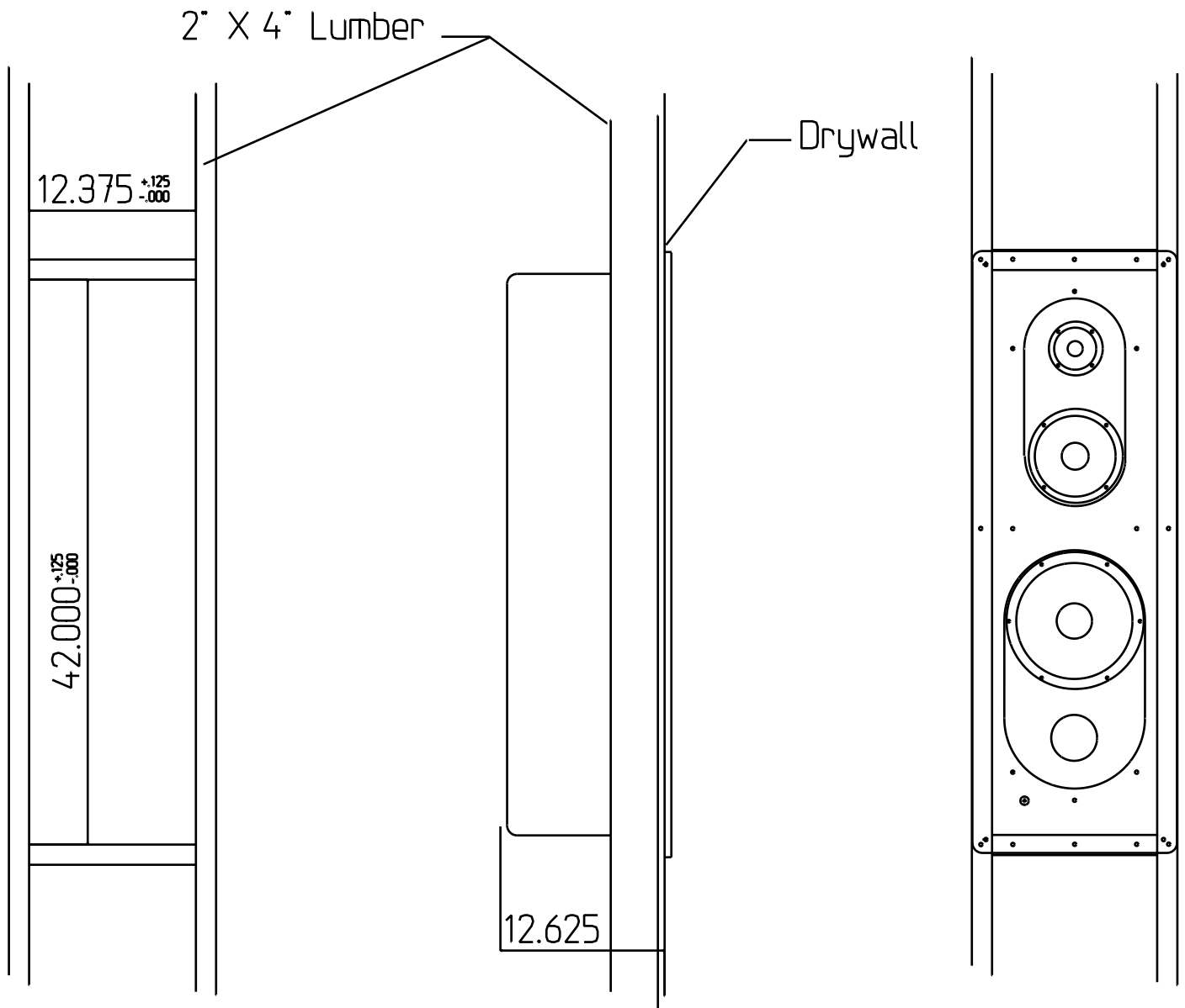
Side View
